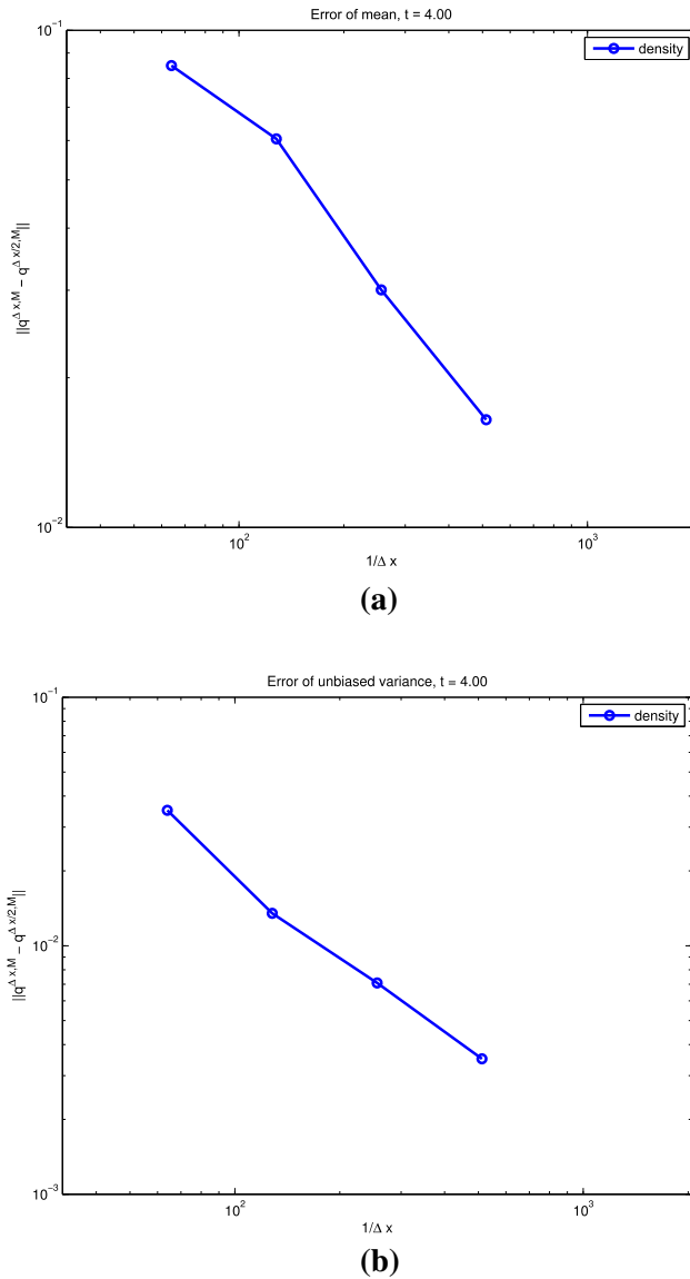
Fig. 23 Cauchy rates (33) for the mean and variance (y-axis) of the Richtmeyer–Meshkov problem (36) at time t = 4 and at different grid resolutions ( x -axis). All results are obtained with 400 Monte Carlo samples. a Mean, b variance
